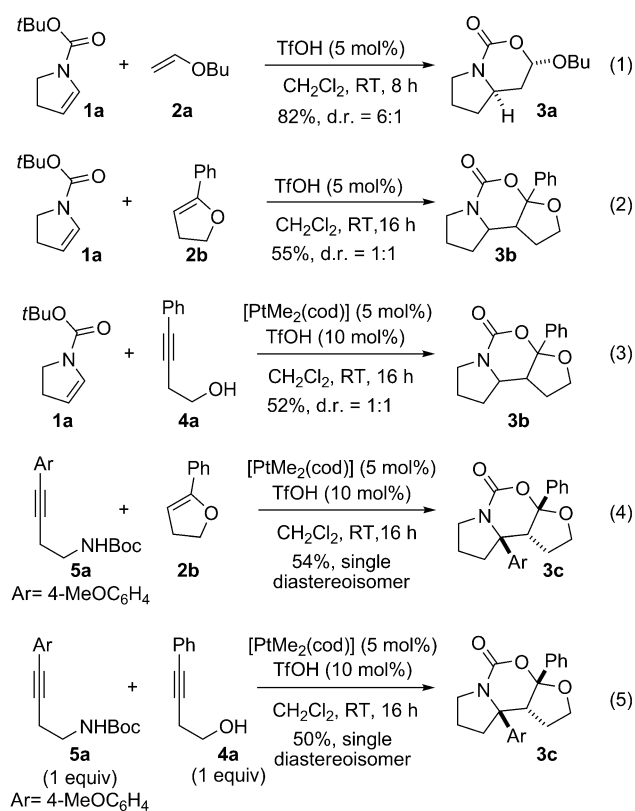
Scheme 2. Initial experiments.
